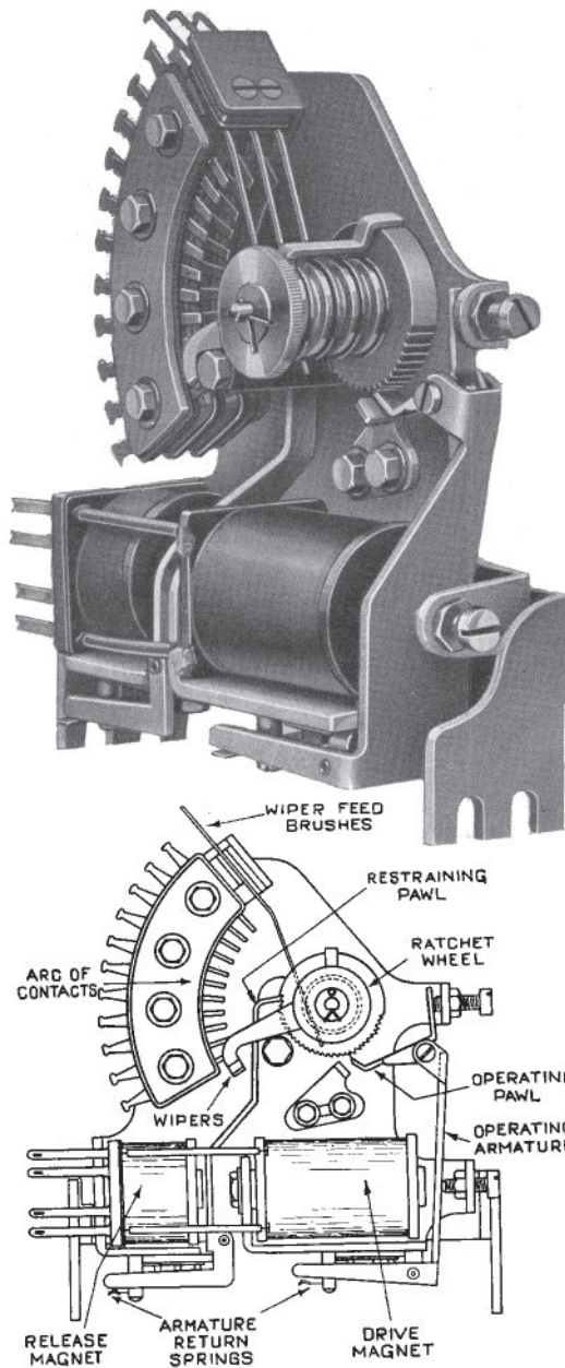
Fig 11. - WAY-STATION SELECTOR
