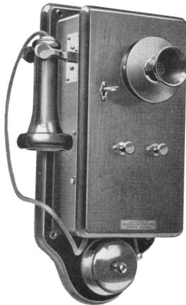
Fig. 1. - WAYSTATION TELEPHONE FOR OMNIBUS CIRCUIT TERMINATED AT A CONTROL OFFICE Telephone shown open for inspection. In this type, carbon lightning arresters are included and a lock is provided to prevent interference by unauthorised persons. (G.E.C.)
