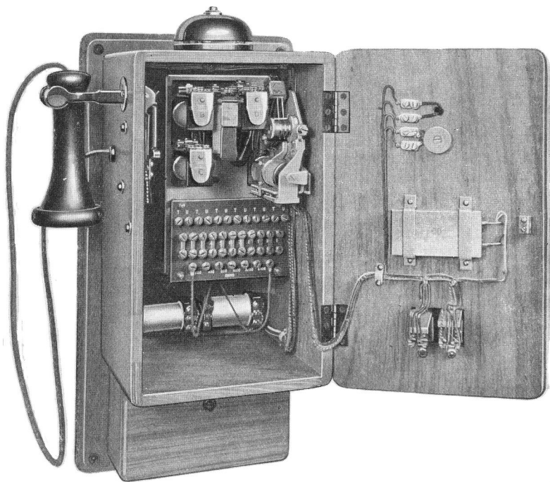
Fig 10 - WAY-STATION TELEPHONE
