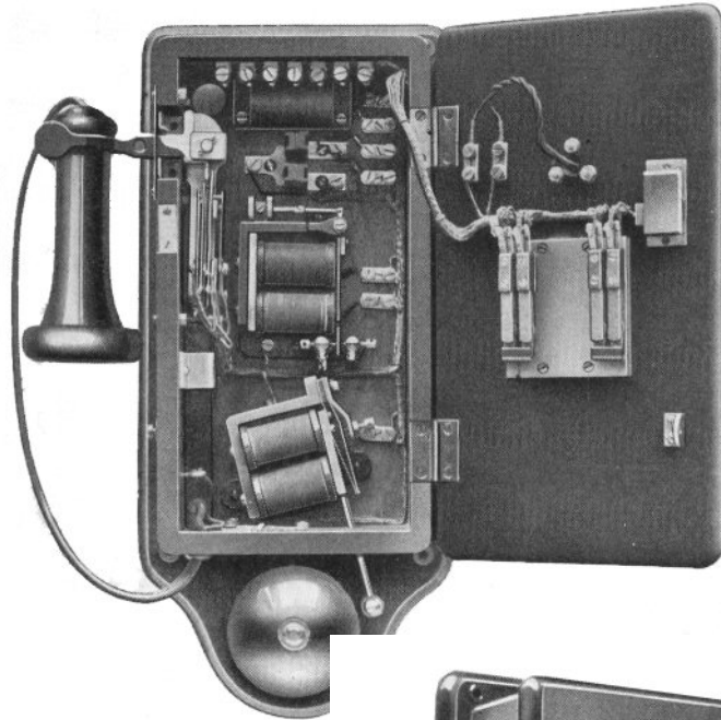
Fig. 1. - WAYSTATION TELEPHONE FOR OMNIBUS CIRCUIT TERMINATED AT A CONTROL OFFICE Telephone shown open for inspection. In this type, carbon lightning arresters are included and a lock is provided to prevent interference by unauthorised persons. (G.E.C.)
